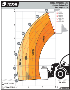
EURO 8 Carriage
